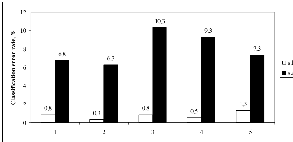
Fig. 5. Classification results obtained using spectra analysis: 1,2,3-training errors: 1-PCA model, 2-Wavelet1+PCA model, 3-Wavelet2+PCA model; 4-validation errors; 5-testing errors: s1-non grain impurities are excluded from validation and testing sets, s2-non grain impurities are included in validation and testing sets
