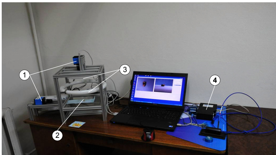
Fig. 1. INTECHN platform hardware components
